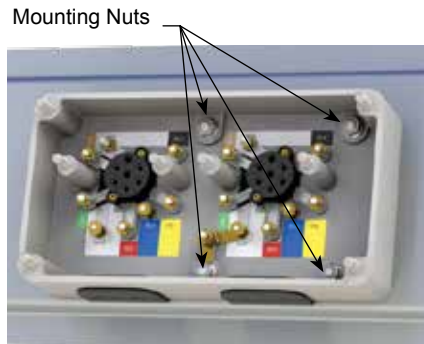
Mounting Nuts
